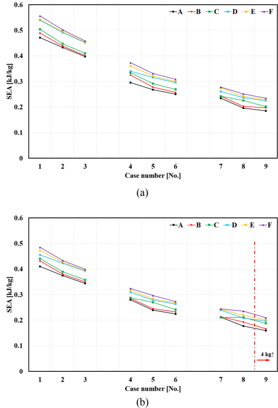
Fig. 7 Comparison with energy absorbed unit per mass: (a) Model 1, (b) Model 2
