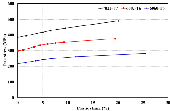
Fig. 4 True stress-strain curves of extruded aluminium
